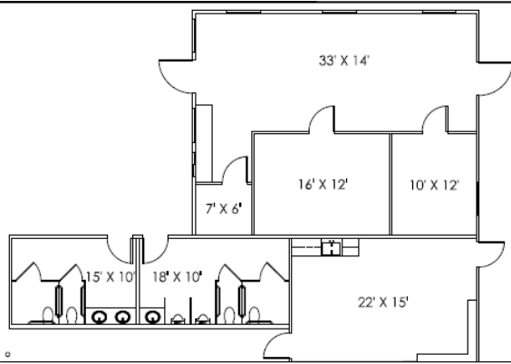
OFFICE PLAN 3/32" = 1'-0"
